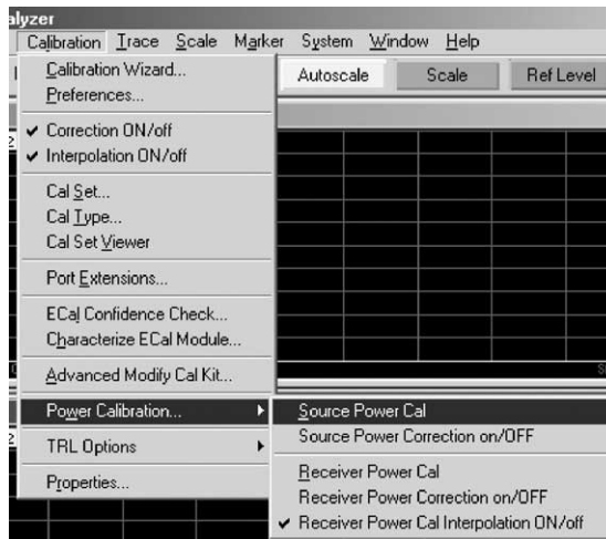
Figure 12. Source power calibration transfers the accuracy of a power meter measurement to the MW PNA source.
