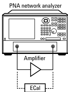
Figure 1. Setup for testing transmission and reflection parameters.
